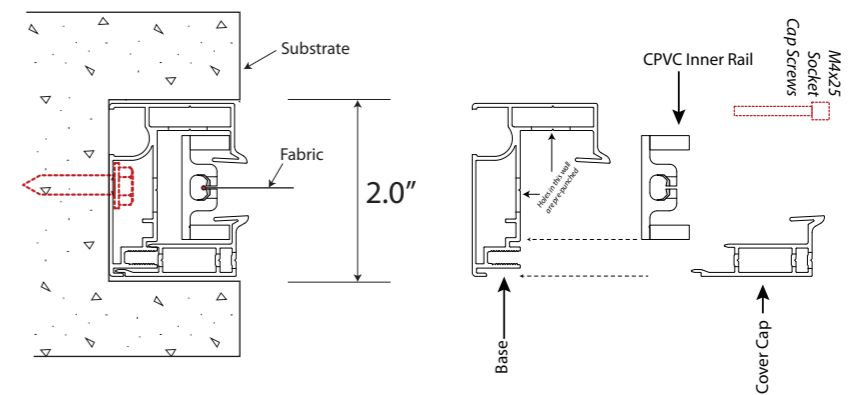
Section A:A of Side Channel (From Above Looking Down):
